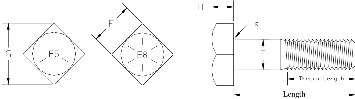
Square Head Bolt Dimensions (per ASME B18.2.1)
